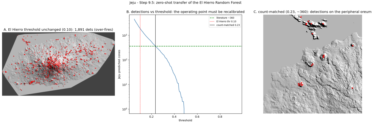
Figure 15: Step 9.5 on Jeju: zero-shot transfer of the El Hierro Random Forest. A : at the unchanged El Hierro threshold the model over-fires ( \sim 1,900 detections). B : detections vs threshold — the operating point must be recalibrated (literature \sim 360 in green, El Hierro threshold in red). C : at the count-matched threshold the detections fall on the peripheral oreum.
