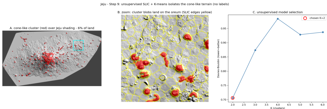
Figure 14: Step 9 on Jeju (no ground truth). A : the unsupervised cone-like cluster (red) over the NE shading, \sim 6\% of the land. B : zoom on a lava plain — the cluster blobs land on the individual oreum (SLIC superpixel edges in yellow). C : Davies–Bouldin model selection picks K = 2 .
